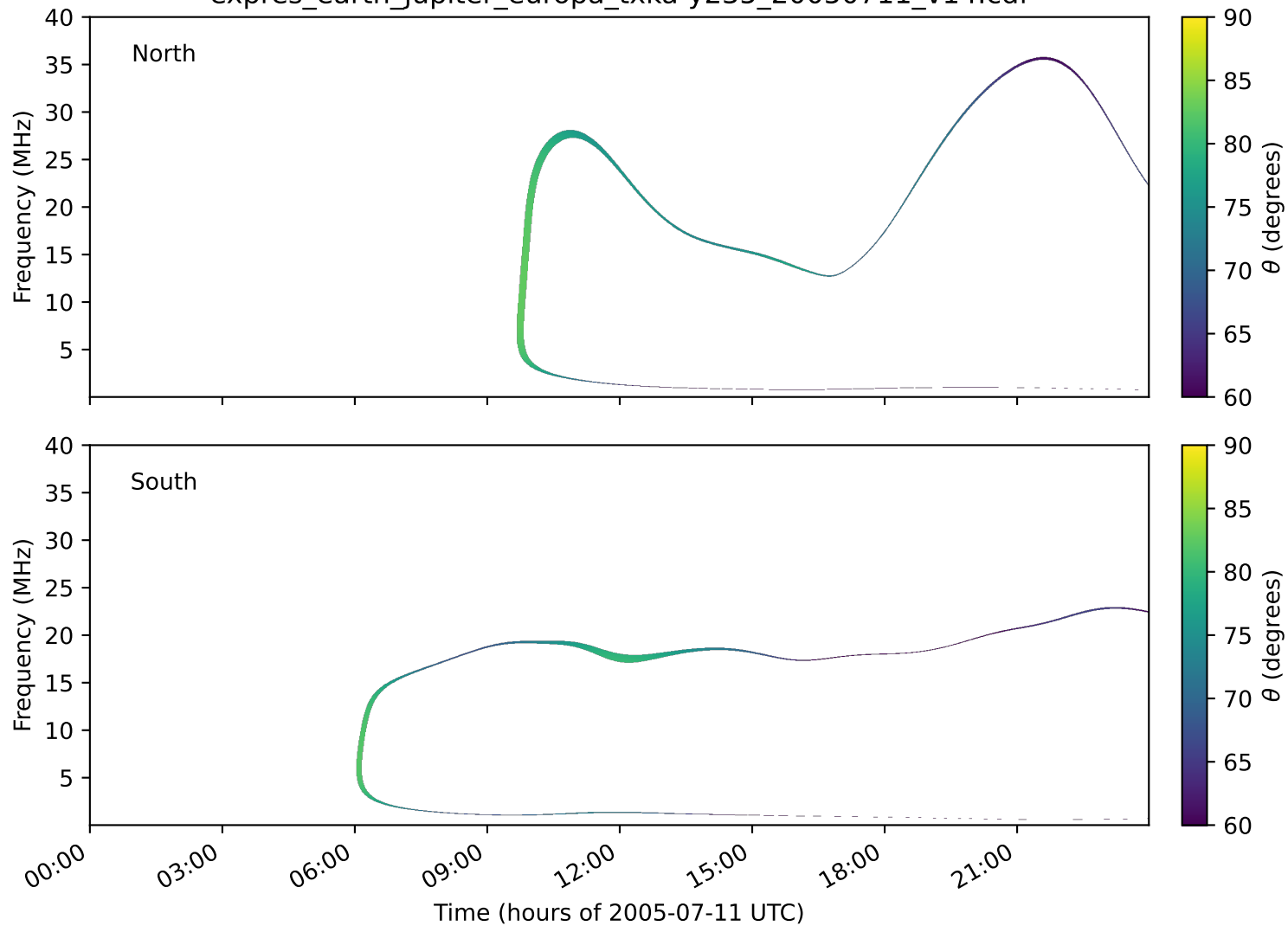
expres_earth_jupiter_europa_txka-y235_20050711_v14.cdf
