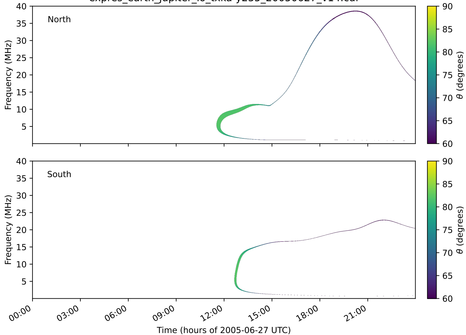
expres_earth_jupiter_io_txka-y235_20050627_v14.cdf
