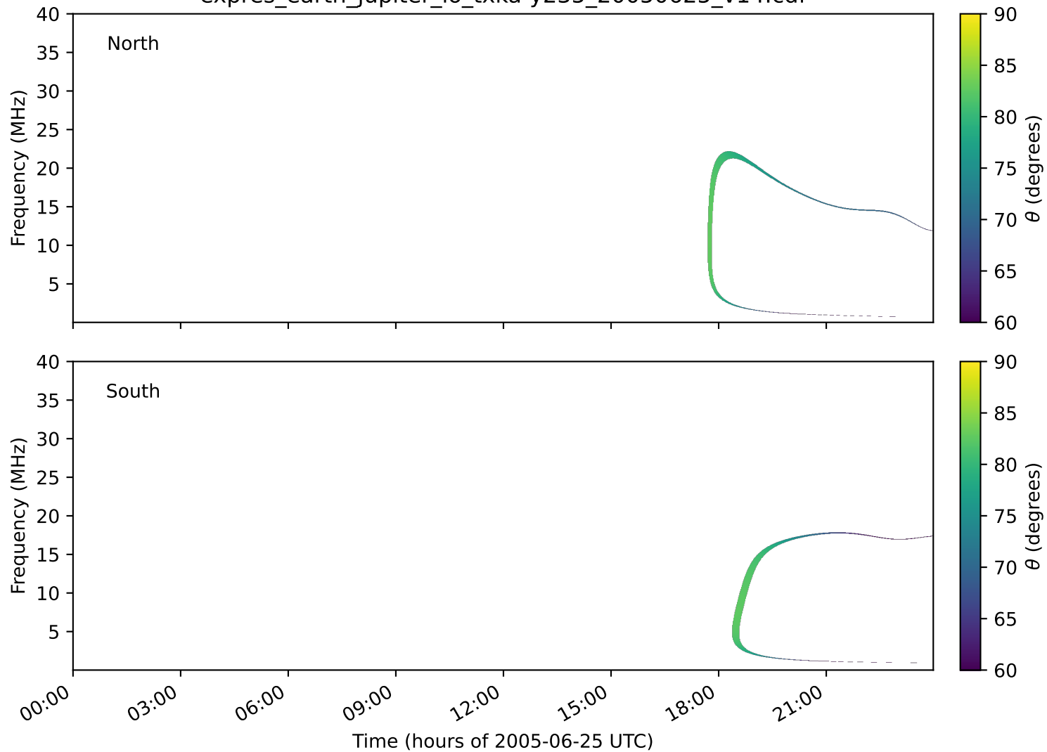
expres_earth_jupiter_io_txka-y235_20050625_v14.cdf
