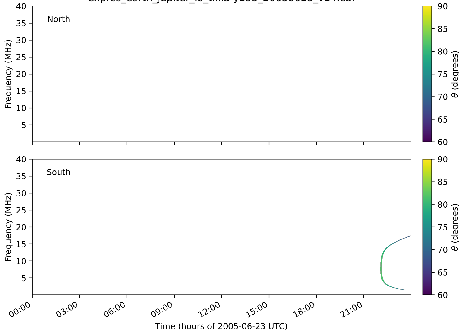
expres_earth_jupiter_io_txka-y235_20050623_v14.cdf
