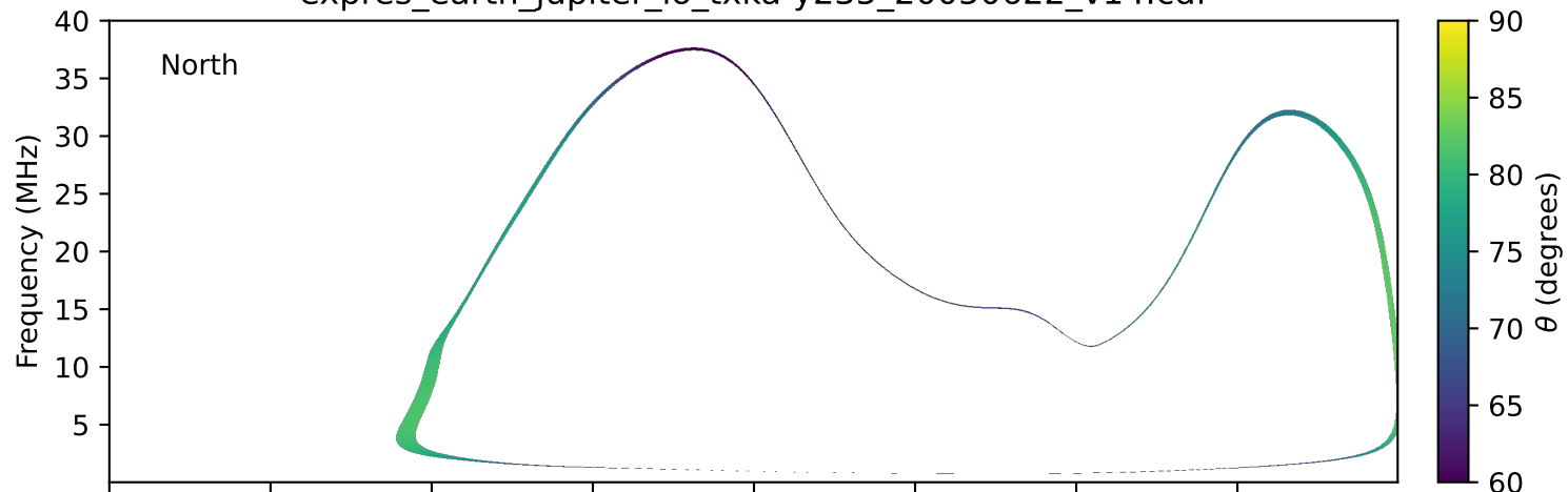
expres_earth_jupiter_io_txka-y235_20050622_v14.cdf
