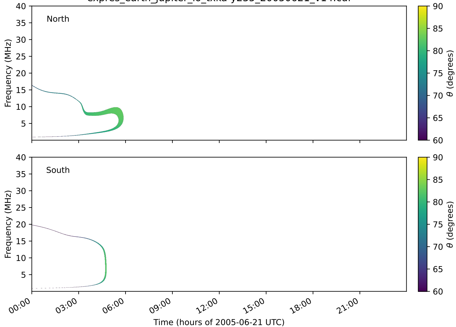
expres_earth_jupiter_io_txka-y235_20050621_v14.cdf
