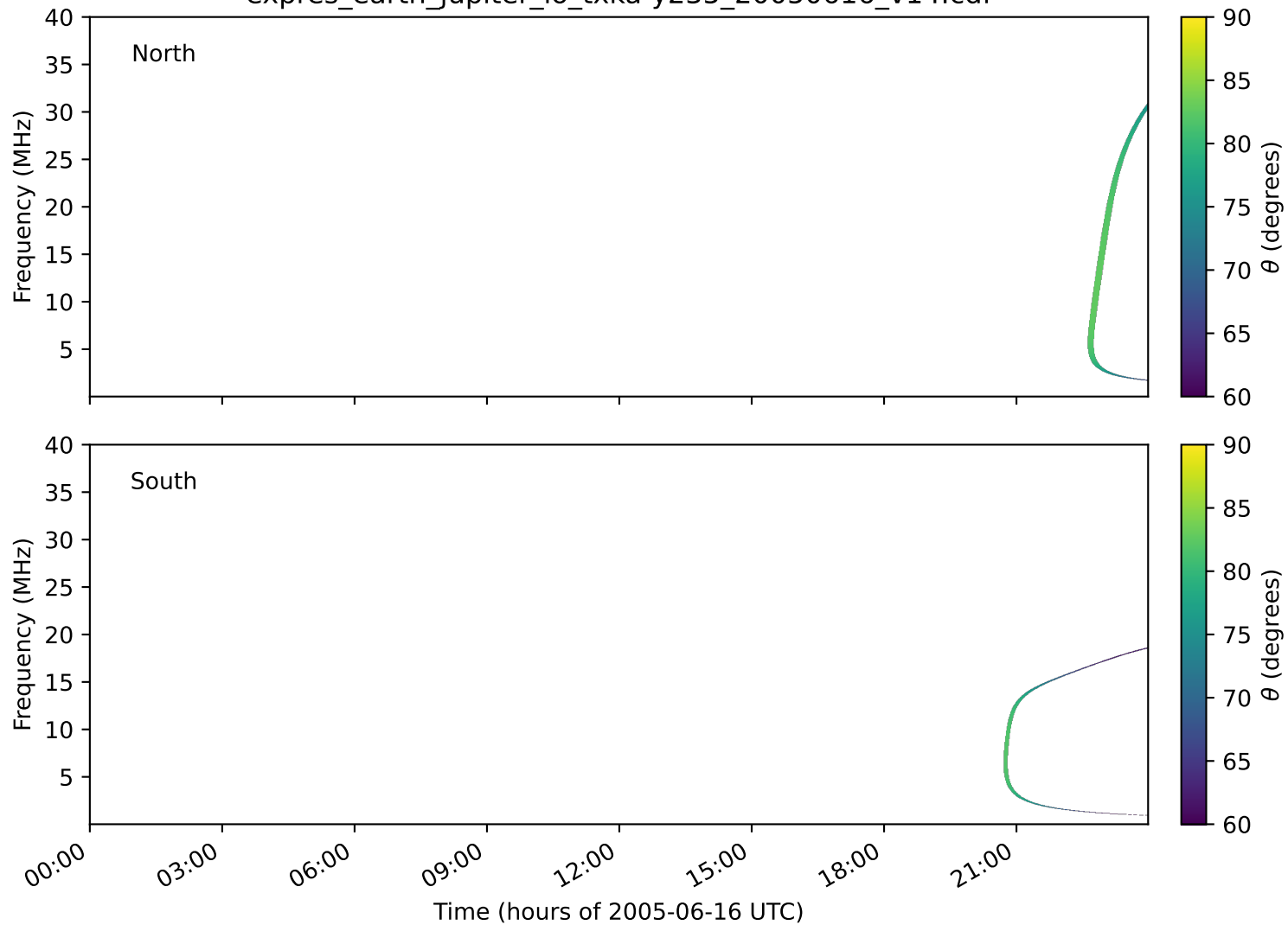
expres_earth_jupiter_io_txka-y235_20050616_v14.cdf
