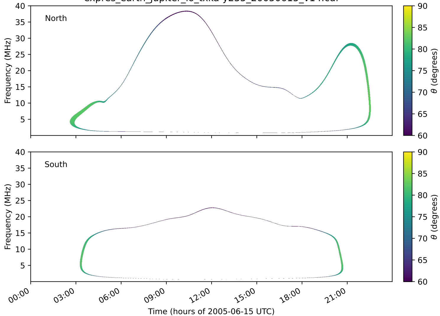
expres_earth_jupiter_io_txka-y235_20050615_v14.cdf
