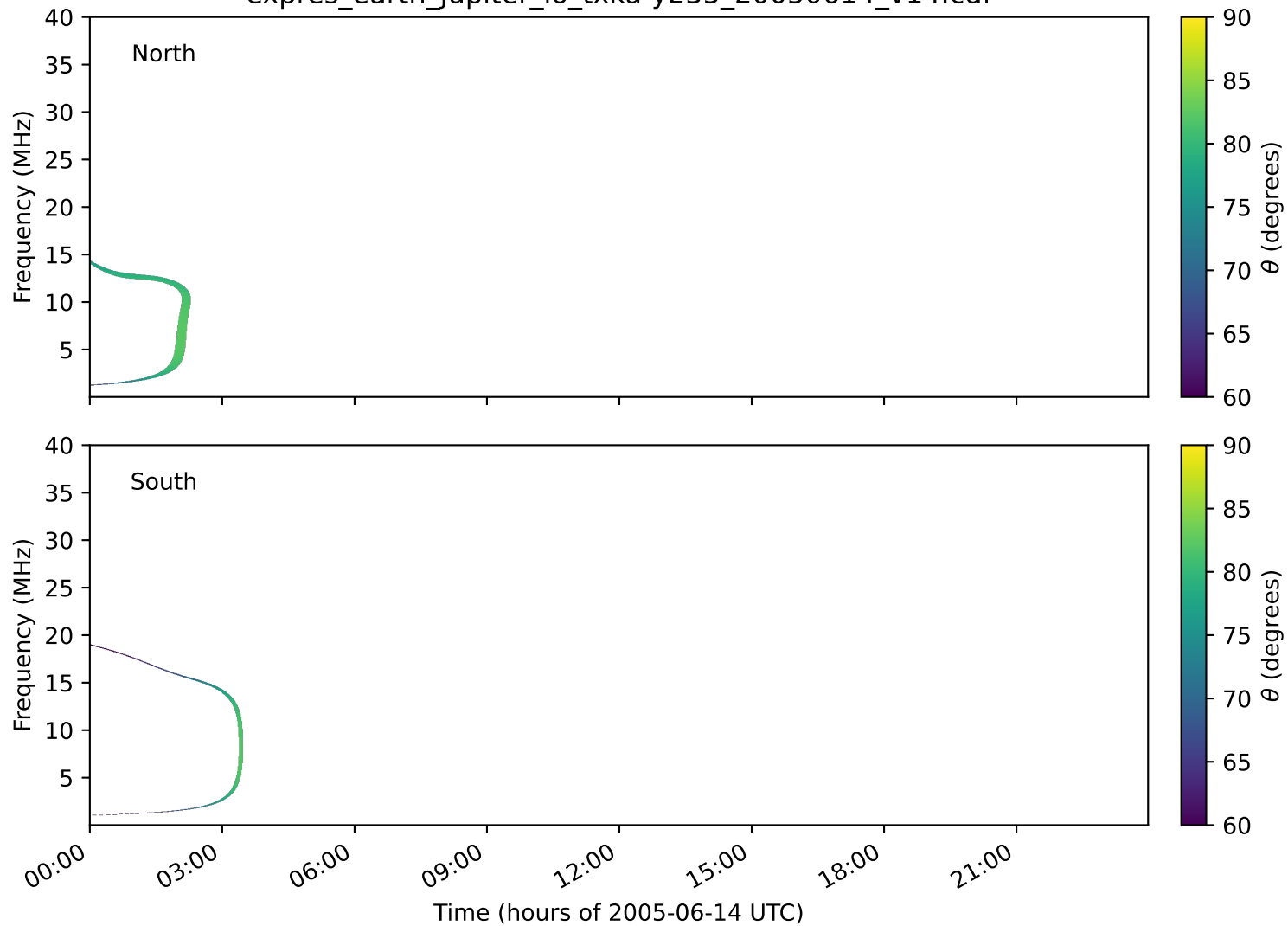
expres_earth_jupiter_io_txka-y235_20050614_v14.cdf
