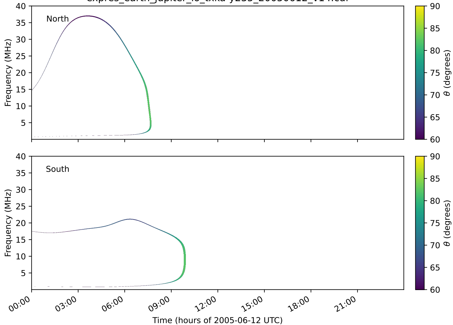
expres_earth_jupiter_io_txka-y235_20050612_v14.cdf
