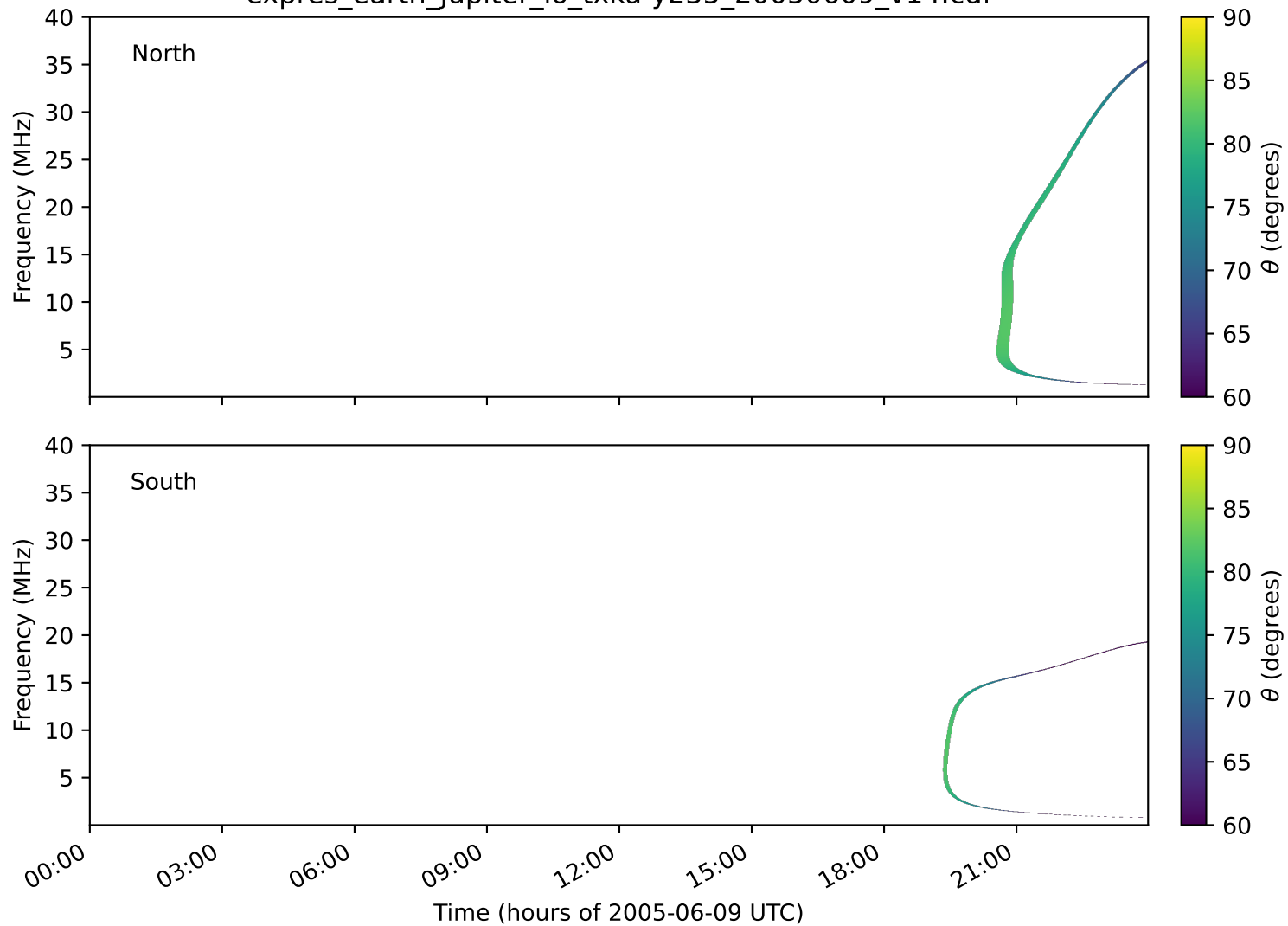
expres_earth_jupiter_io_txka-y235_20050609_v14.cdf
