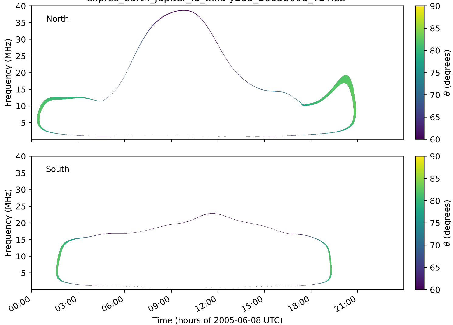
expres_earth_jupiter_io_txka-y235_20050608_v14.cdf
