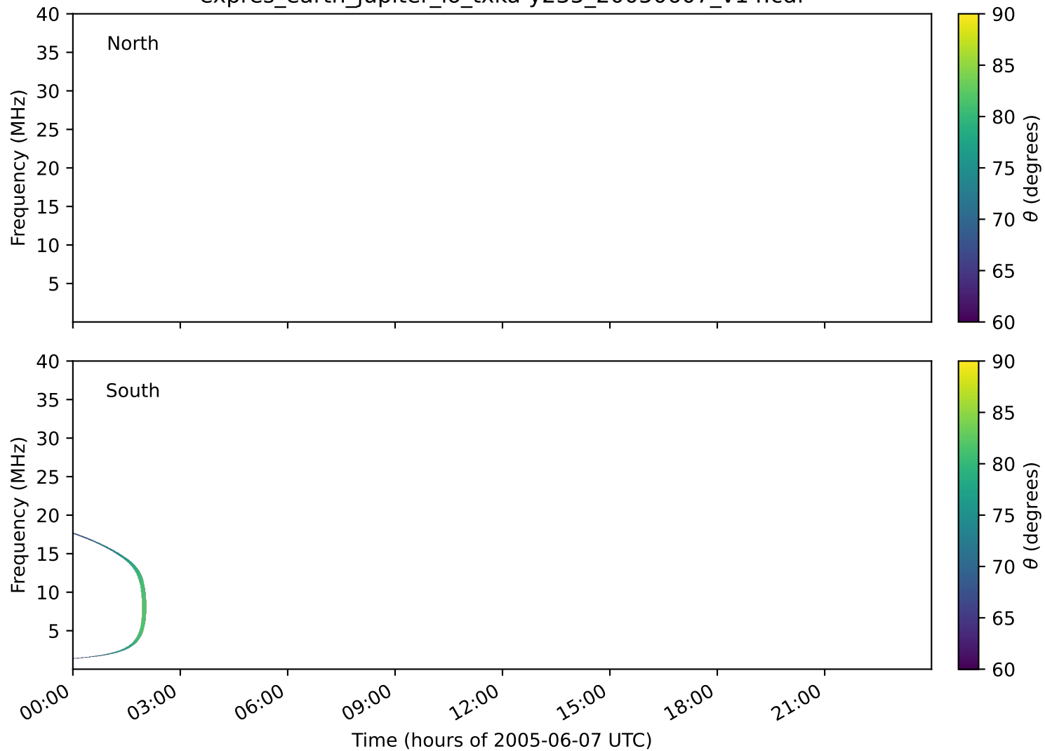
expres_earth_jupiter_io_txka-y235_20050607_v14.cdf
