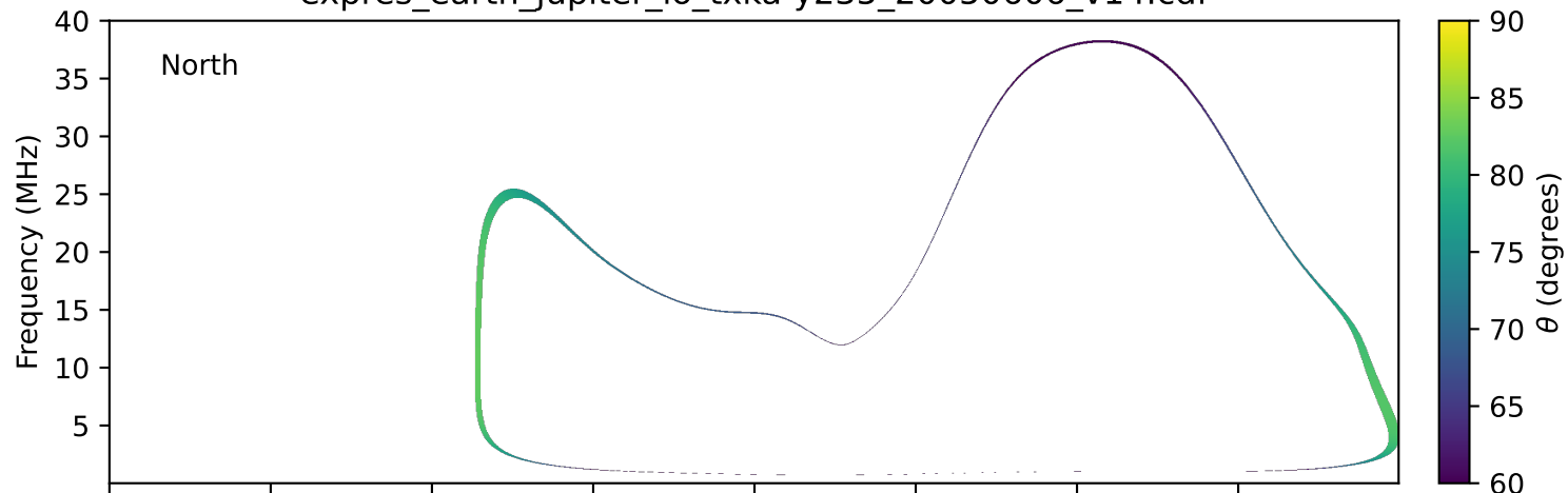
expres_earth_jupiter_io_txka-y235_20050606_v14.cdf
