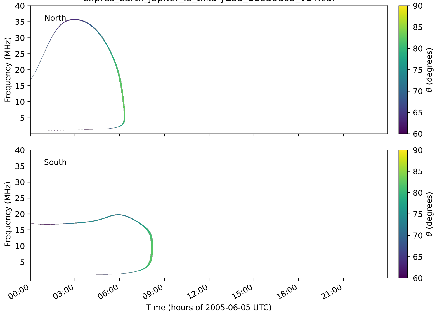
expres_earth_jupiter_io_txka-y235_20050605_v14.cdf
