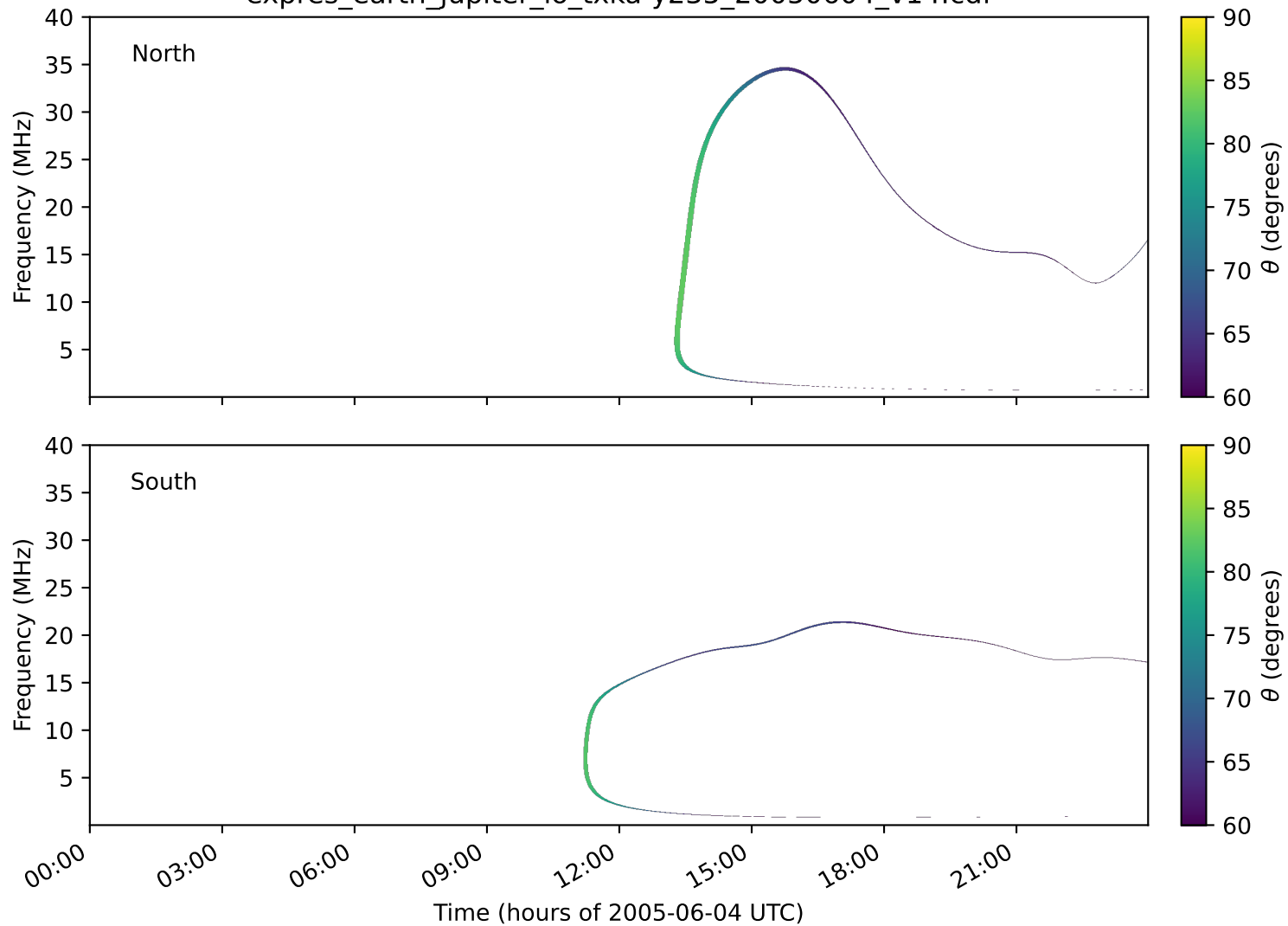
expres_earth_jupiter_io_txka-y235_20050604_v14.cdf
