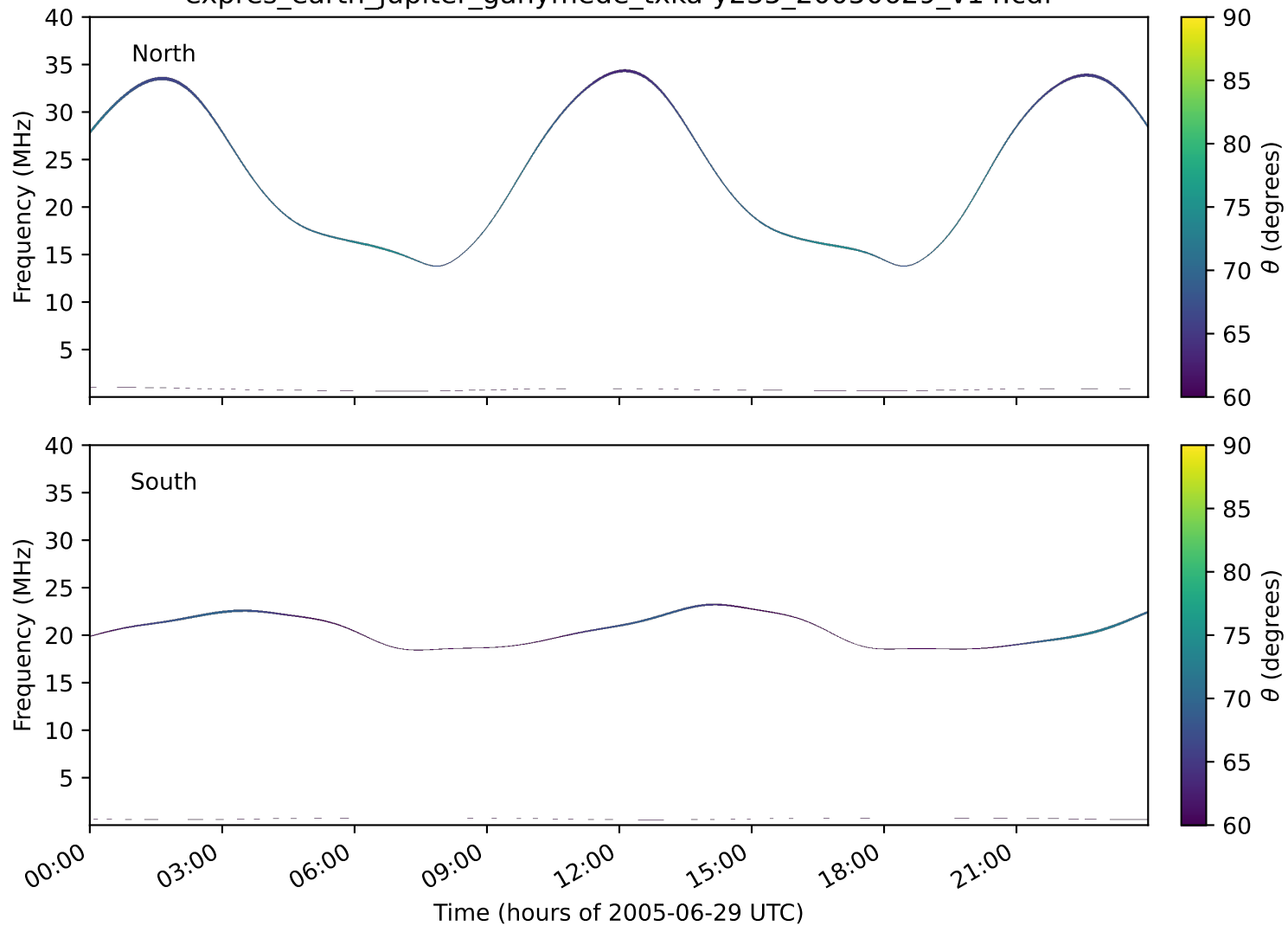
expres_earth_jupiter_ganymede_txka-y235_20050629_v14.cdf
