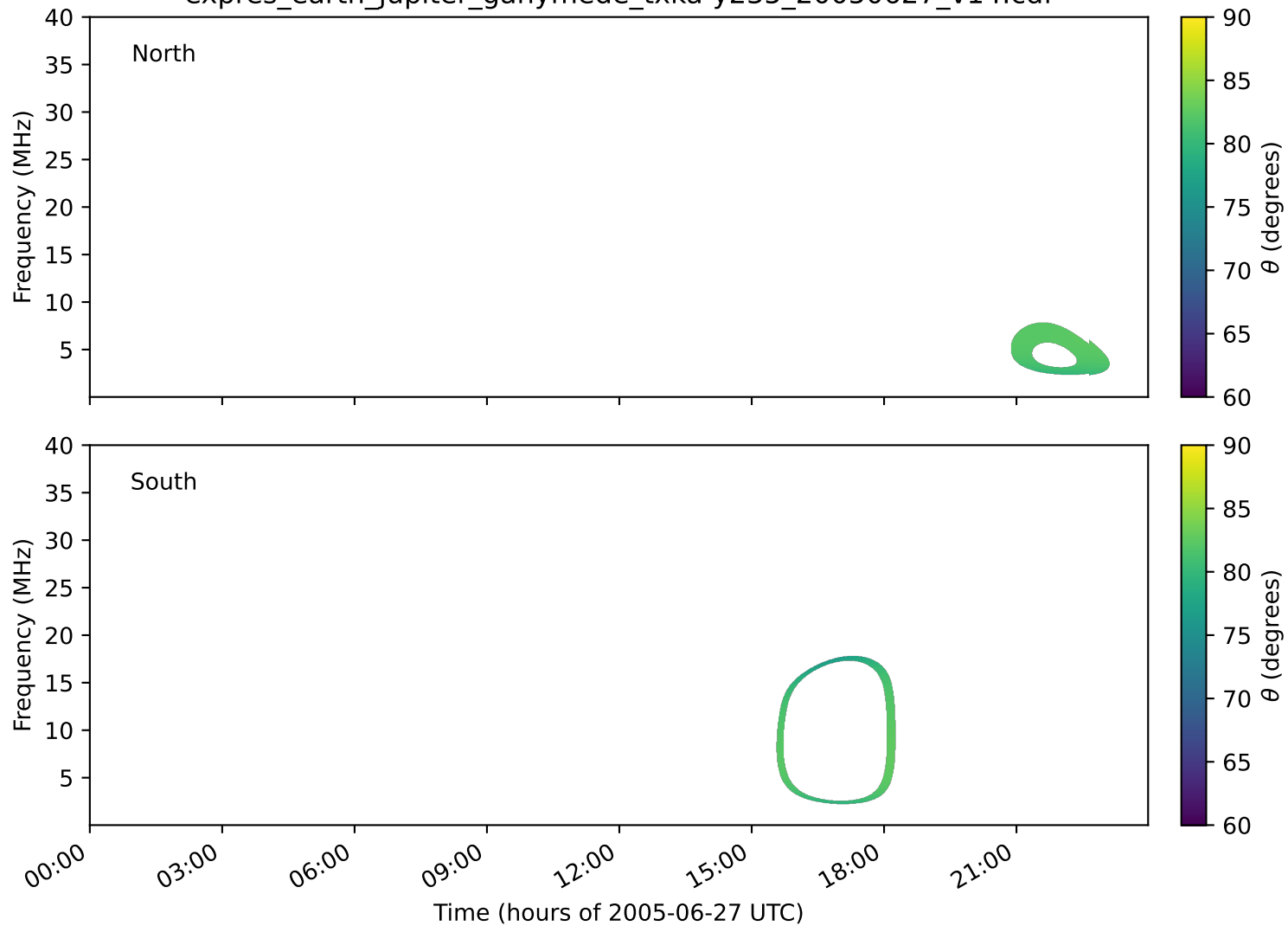
expres_earth_jupiter_ganymede_txka-y235_20050627_v14.cdf
