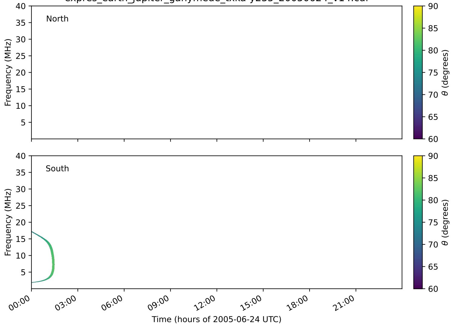
expres_earth_jupiter_ganymede_txka-y235_20050624_v14.cdf
