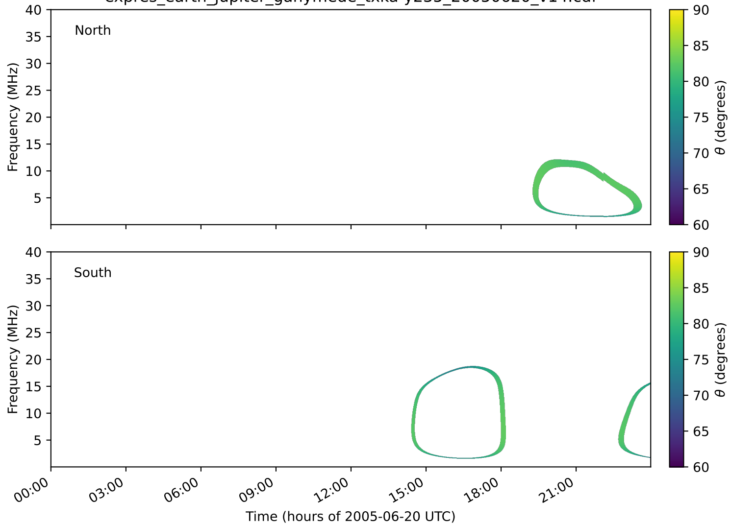
expres_earth_jupiter_ganymede_txka-y235_20050620_v14.cdf
