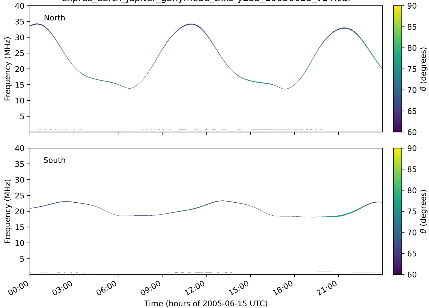
expres_earth_jupiter_ganymede_txka-y235_20050615_v14.cdf
