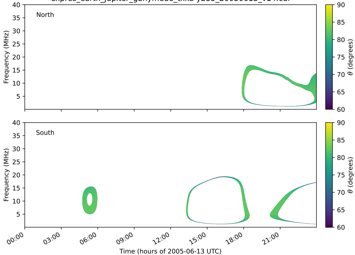
expres_earth_jupiter_ganymede_txka-y235_20050613_v14.cdf
