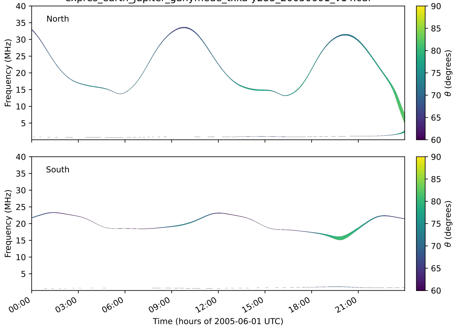
expres_earth_jupiter_ganymede_txka-y235_20050601_v14.cdf
