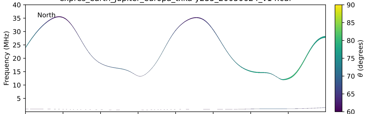
expres_earth_jupiter_europa_txka-y235_20050624_v14.cdf
