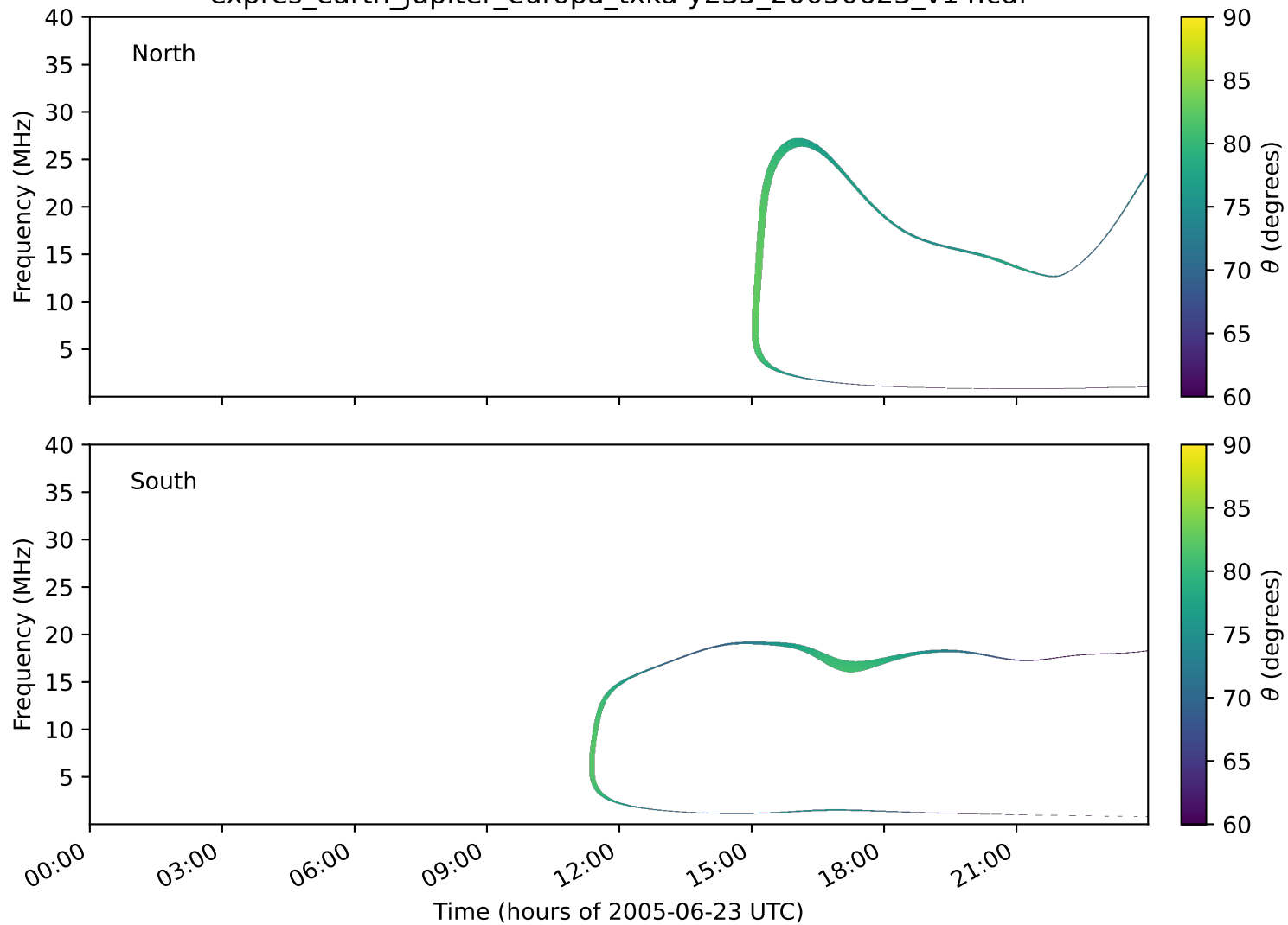
expres_earth_jupiter_europa_txka-y235_20050623_v14.cdf
