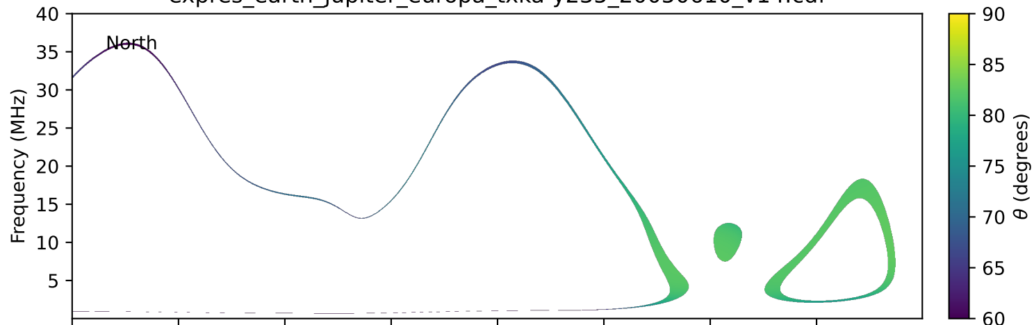
expres_earth_jupiter_europa_txka-y235_20050610_v14.cdf
