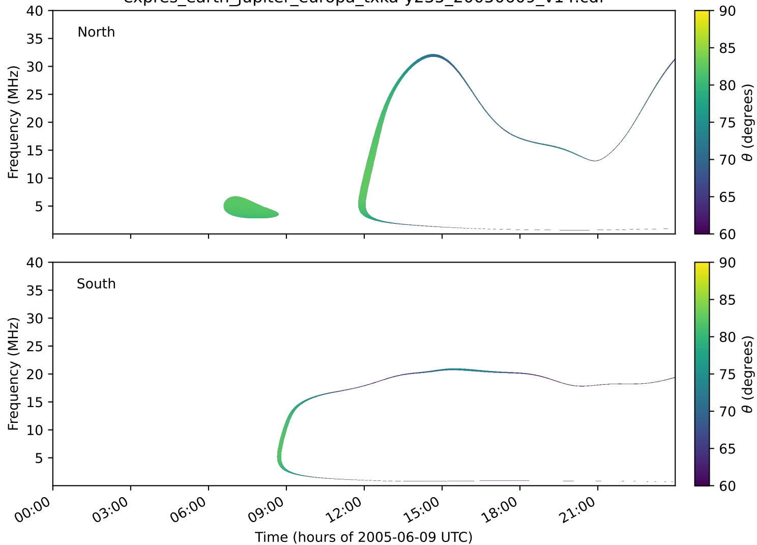
expres_earth_jupiter_europa_txka-y235_20050609_v14.cdf
