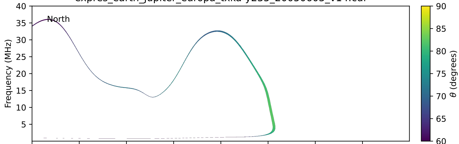
expres_earth_jupiter_europa_txka-y235_20050603_v14.cdf
