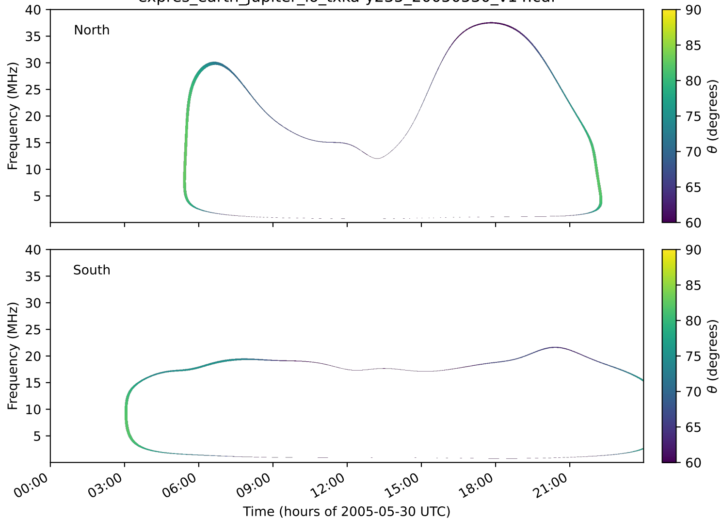
expres_earth_jupiter_io_txka-y235_20050530_v14.cdf
