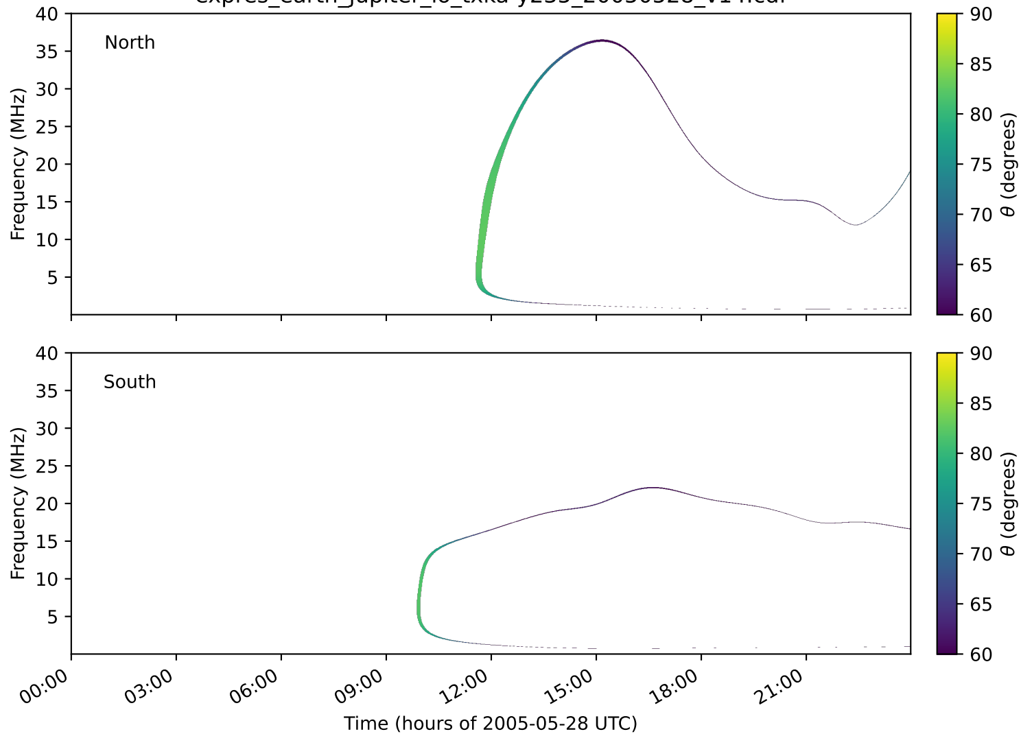
expres_earth_jupiter_io_txka-y235_20050528_v14.cdf
