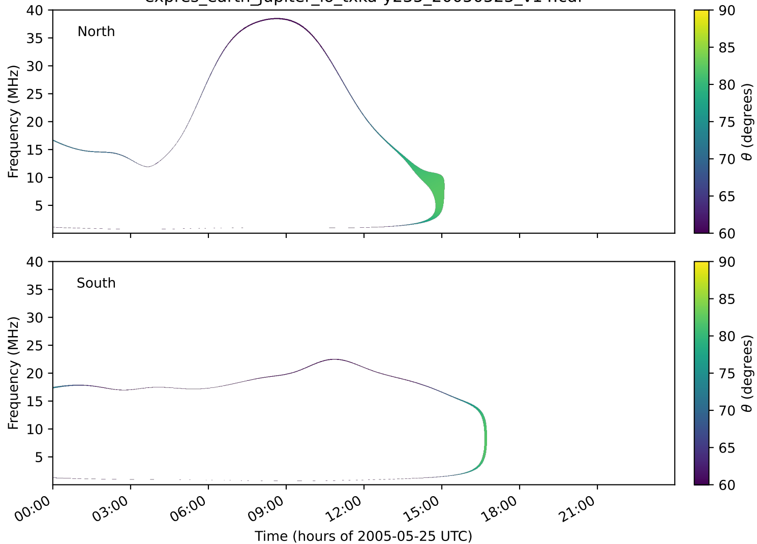
expres_earth_jupiter_io_txka-y235_20050525_v14.cdf
