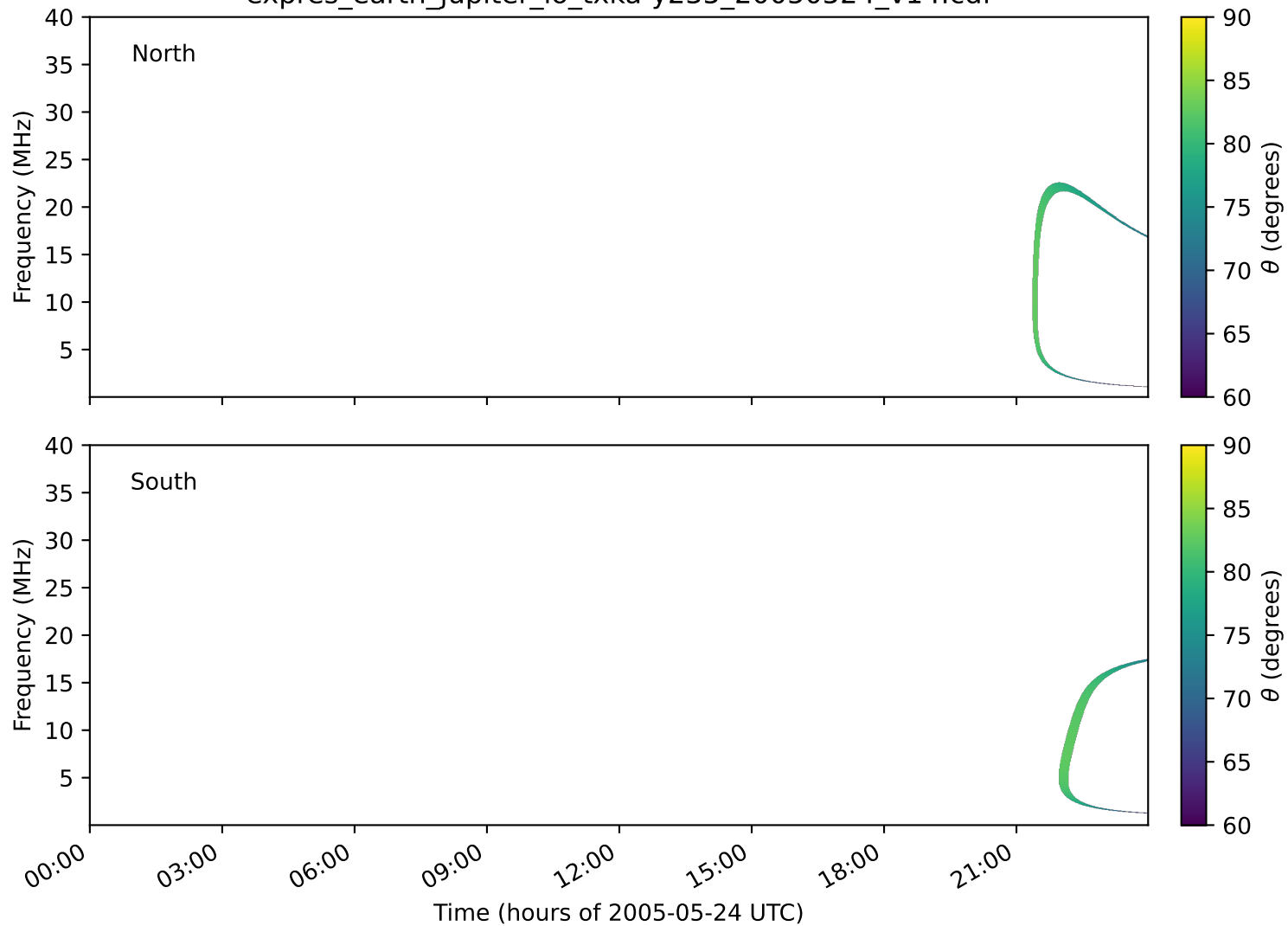
expres_earth_jupiter_io_txka-y235_20050524_v14.cdf
