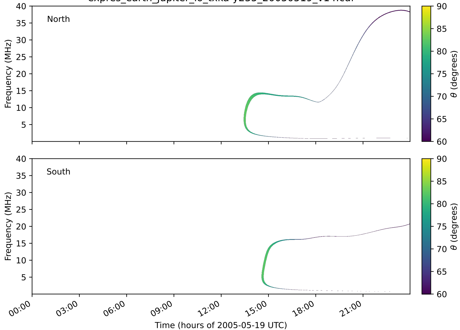
expres_earth_jupiter_io_txka-y235_20050519_v14.cdf
