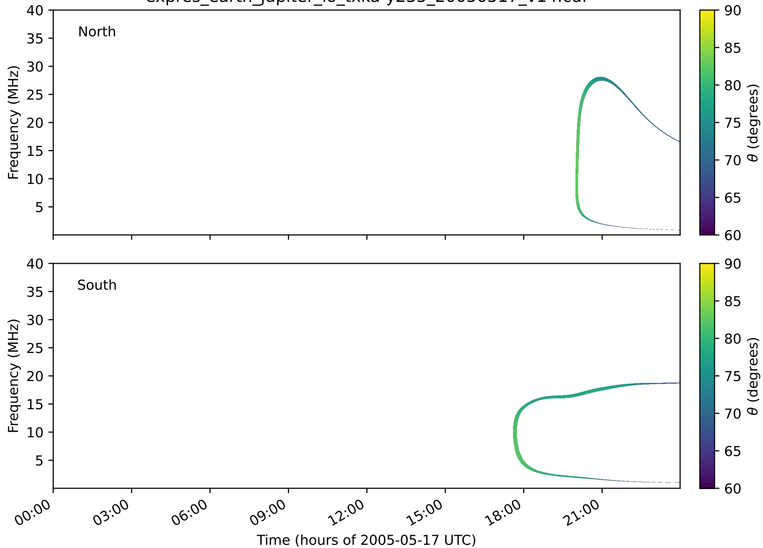
expres_earth_jupiter_io_txka-y235_20050517_v14.cdf
