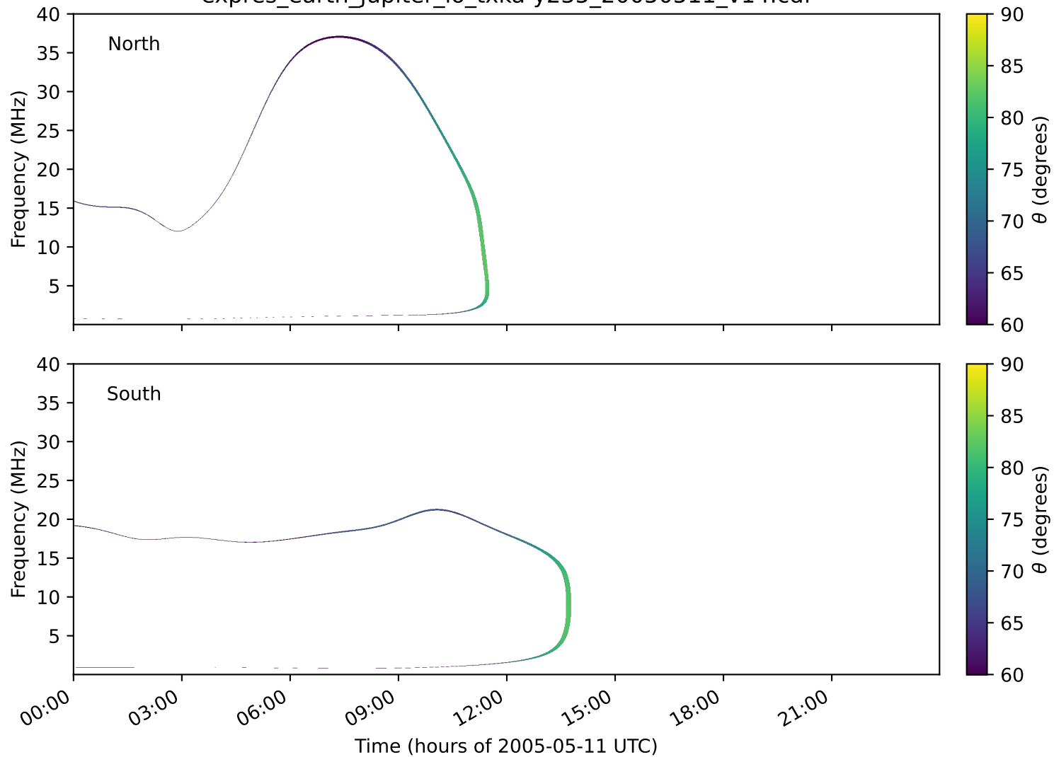
expres_earth_jupiter_io_txka-y235_20050511_v14.cdf
