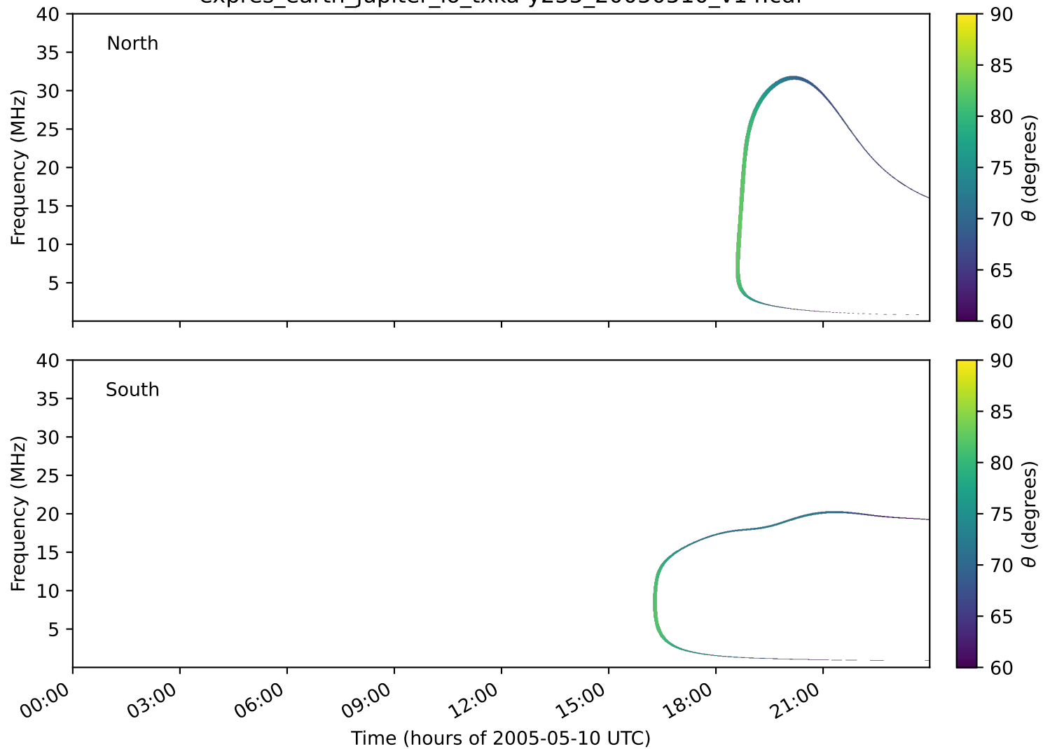
expres_earth_jupiter_io_txka-y235_20050510_v14.cdf
