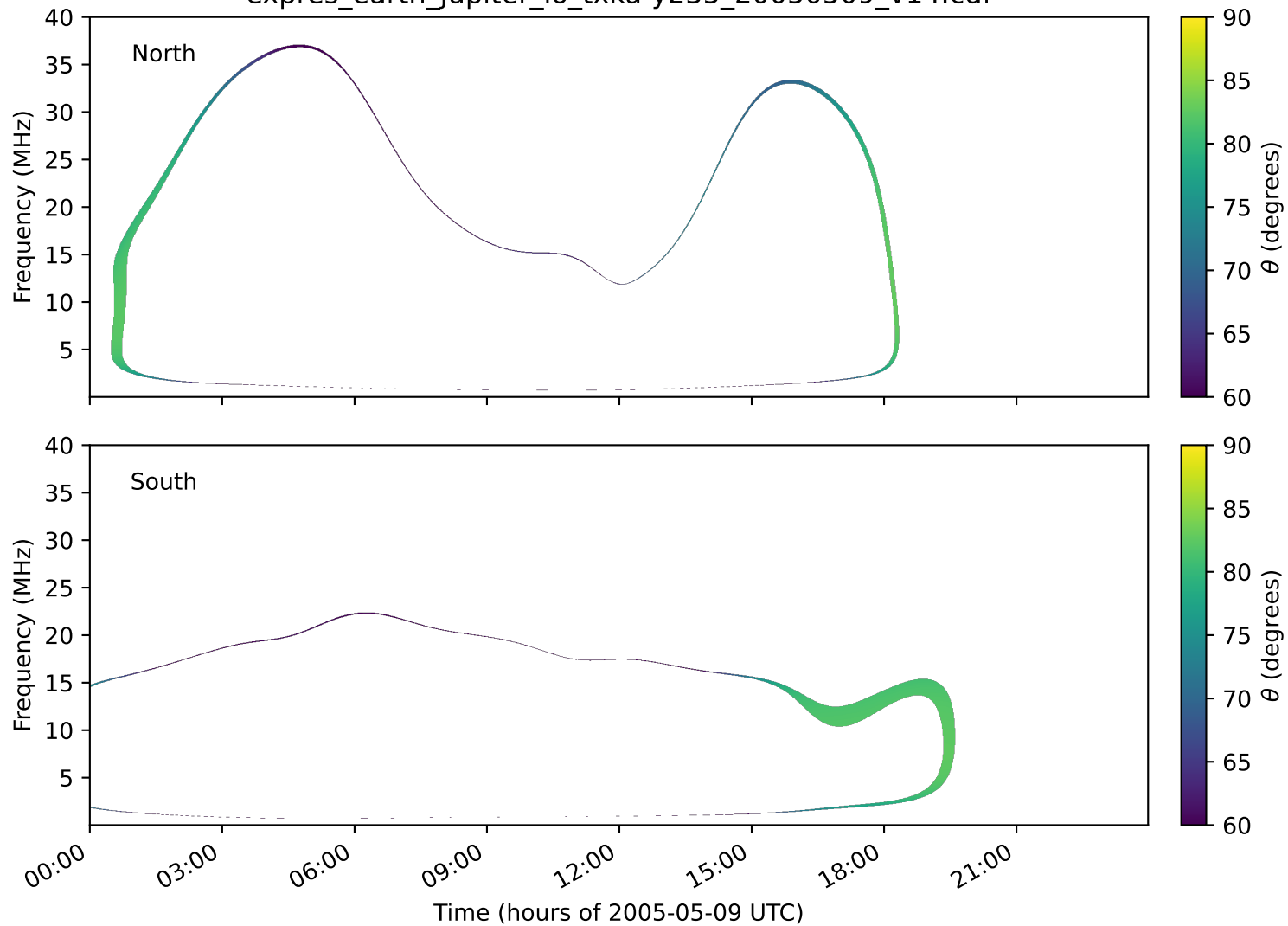
expres_earth_jupiter_io_txka-y235_20050509_v14.cdf
