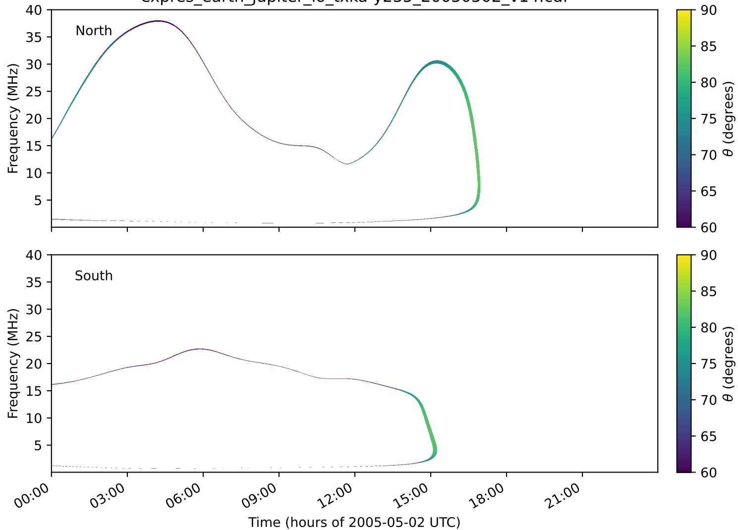
expres_earth_jupiter_io_txka-y235_20050502_v14.cdf
