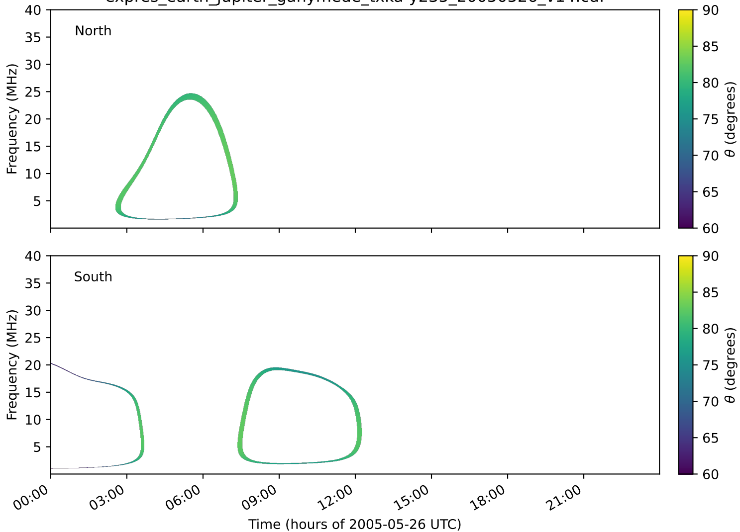
expres_earth_jupiter_ganymede_txka-y235_20050526_v14.cdf
