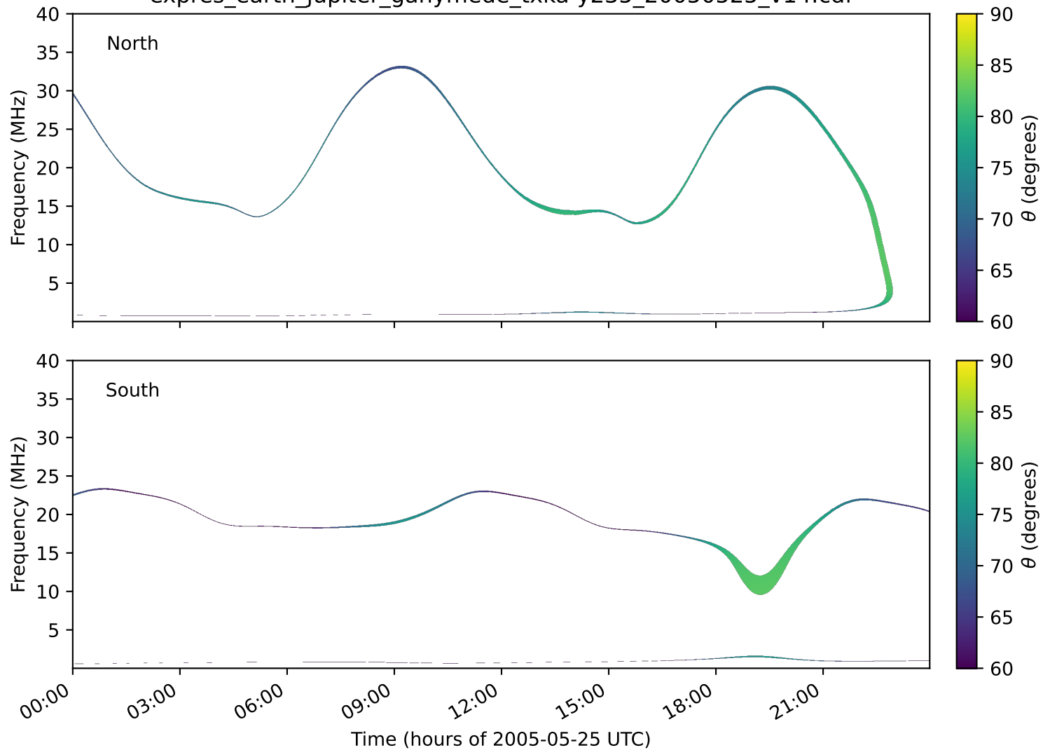
expres_earth_jupiter_ganymede_txka-y235_20050525_v14.cdf
