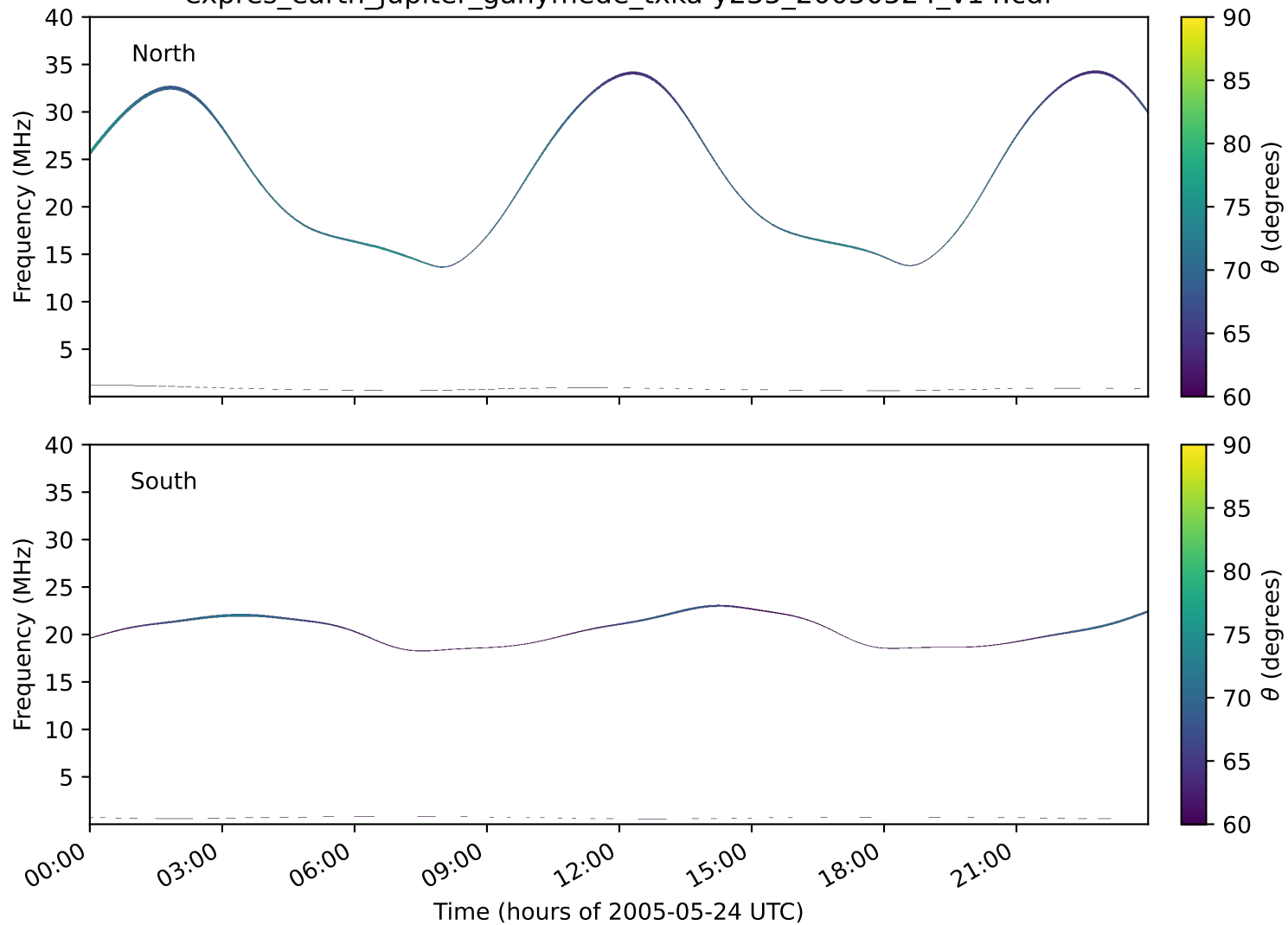
expres_earth_jupiter_ganymede_txka-y235_20050524_v14.cdf
