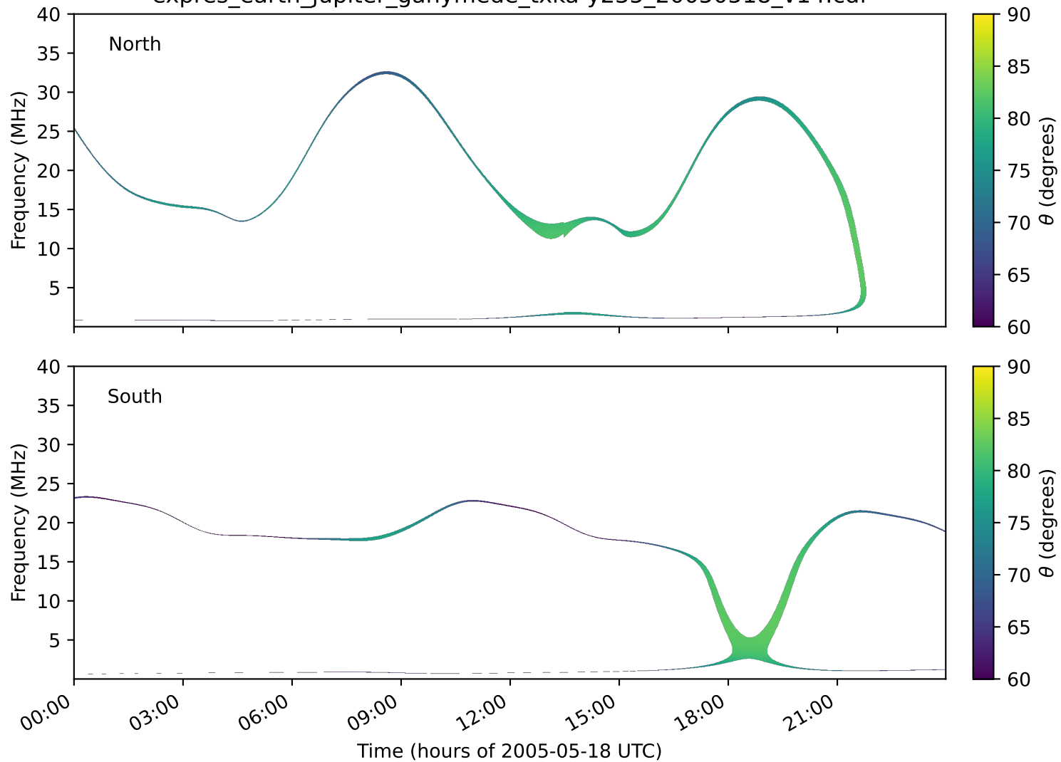
expres_earth_jupiter_ganymede_txka-y235_20050518_v14.cdf
