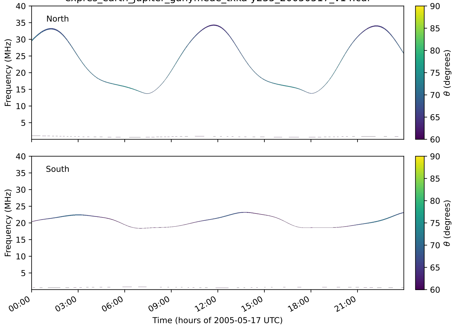
expres_earth_jupiter_ganymede_txka-y235_20050517_v14.cdf
