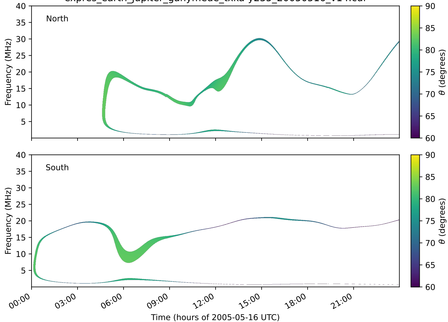
expres_earth_jupiter_ganymede_txka-y235_20050516_v14.cdf
