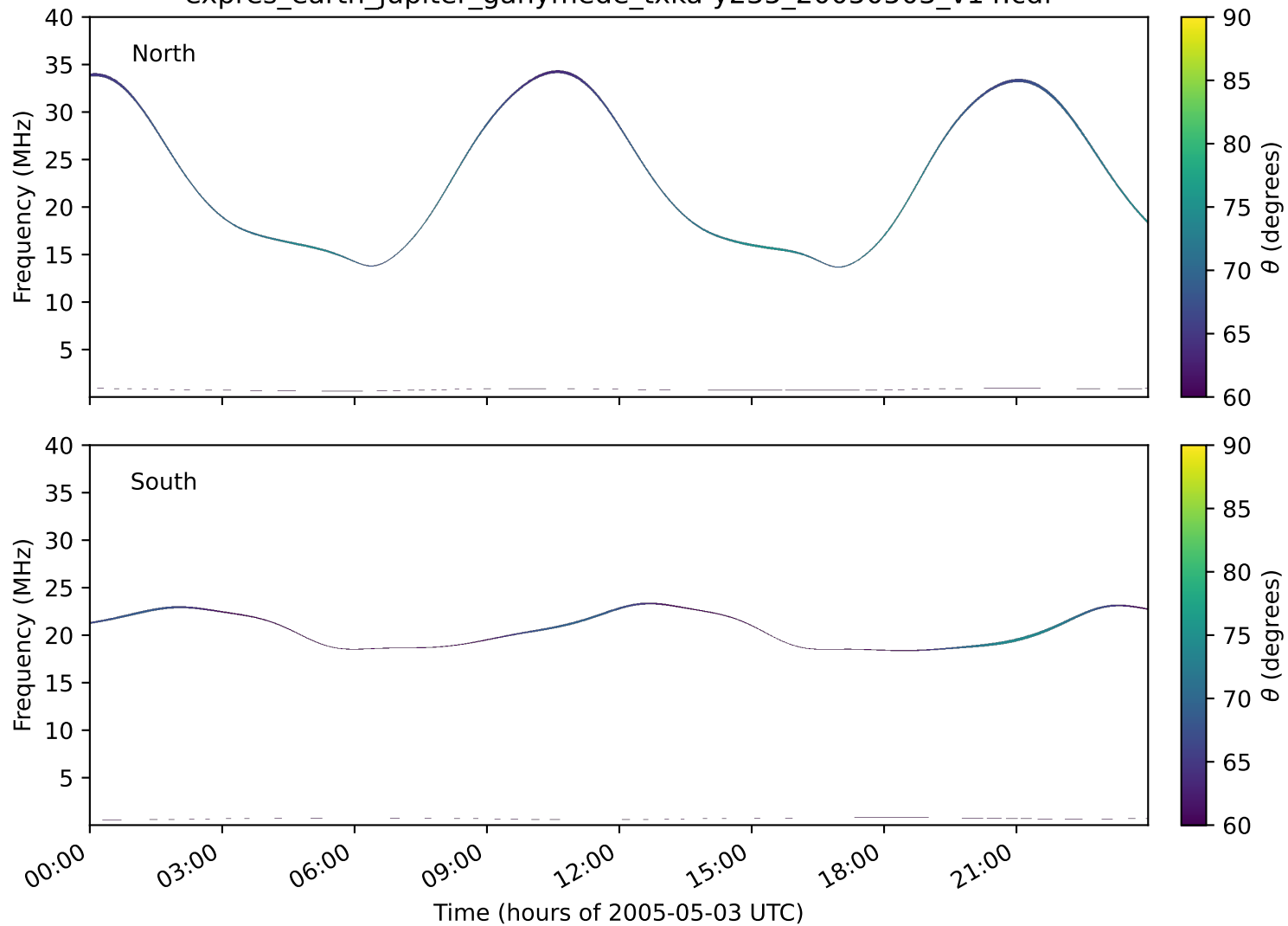
expres_earth_jupiter_ganymede_txka-y235_20050503_v14.cdf
