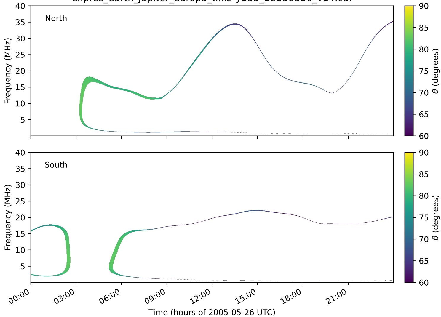
expres_earth_jupiter_europa_txka-y235_20050526_v14.cdf
