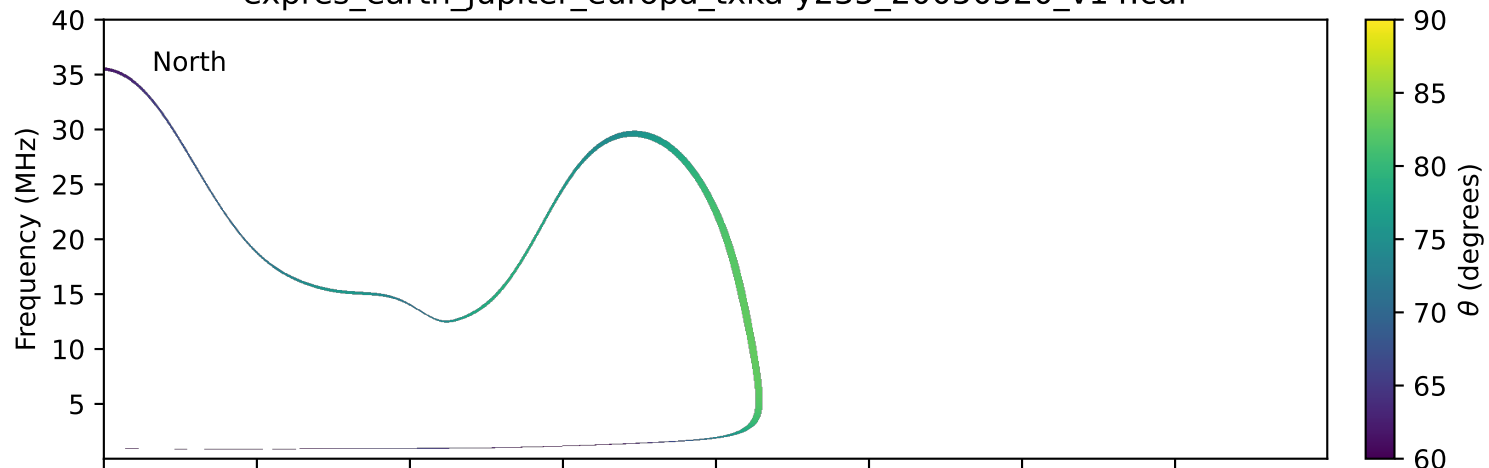
expres_earth_jupiter_europa_txka-y235_20050520_v14.cdf
