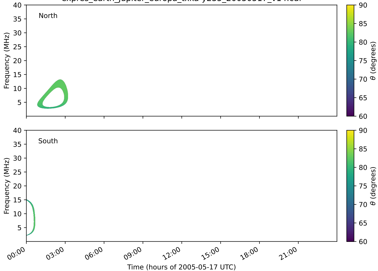
expres_earth_jupiter_europa_txka-y235_20050517_v14.cdf
