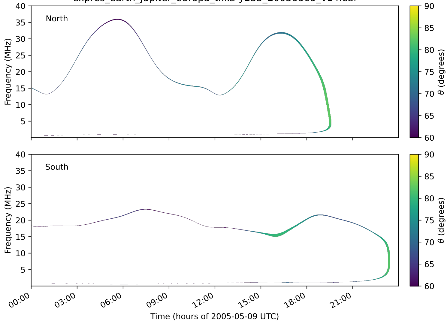
expres_earth_jupiter_europa_txka-y235_20050509_v14.cdf
