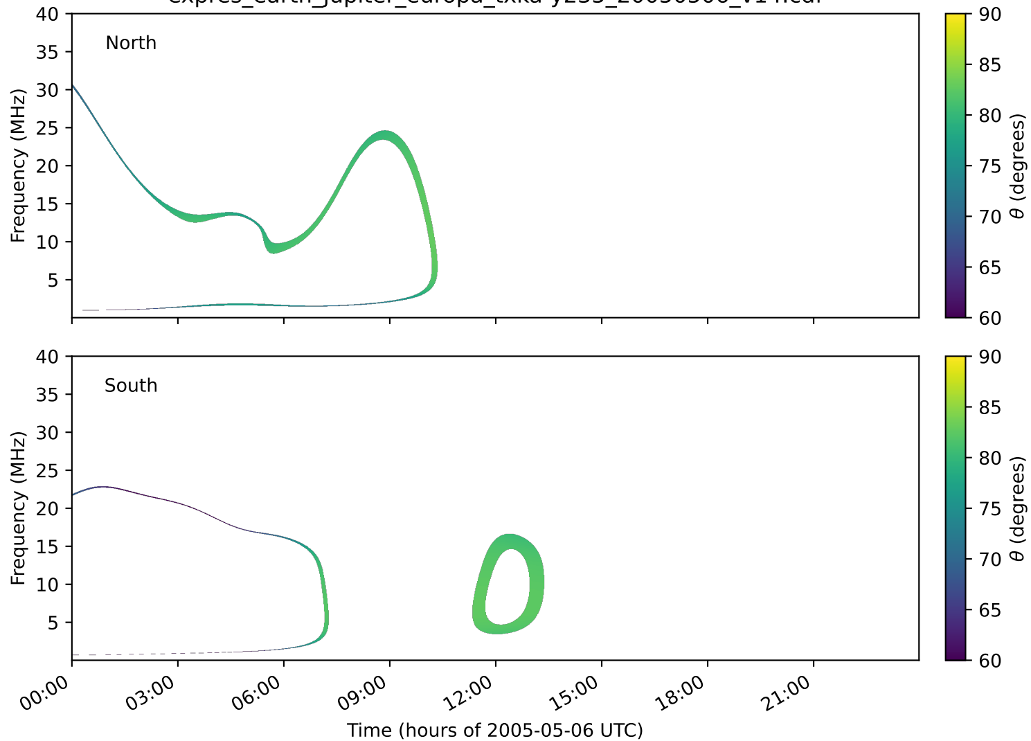
expres_earth_jupiter_europa_txka-y235_20050506_v14.cdf
